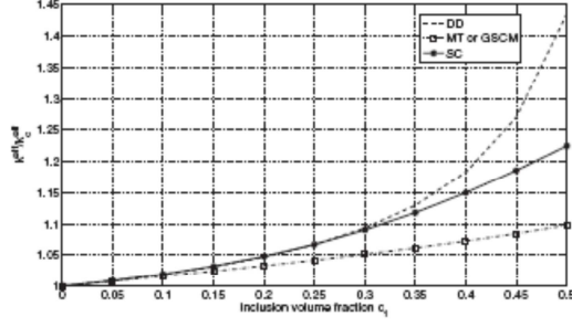
FIG. 10. The ratio k_s^{eff}/k_c^{eff} versus the inclusion volume fraction c_1 with inclusion radius R=20 \mu\text{m} .
