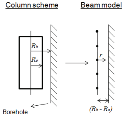
Figure 3: Scheme of the radial displacement.
