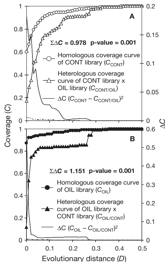
Fig. 1. Results of LIBSHUFF comparisons. (A) Control sediment (CONT) library (X) vs. oiled sediment (OIL) library (Y) and (B) OIL library (Y) vs. CONT library (X). In each case, homologous curve ( C_X , C_Y , circle), heterologous curve ( C_{XY} , C_{YX} , triangle), and \Delta C ( [C_X - C_{XY}]^2 , [C_Y - C_{YX}]^2 , solid line) are presented as a function of evolutionary distance ( D ). For each comparison, \Sigma\Delta C and the corresponding p -value (corresponding to the rank of \Sigma\Delta C within the entire list of the 999 shuffled samples \Sigma\Delta C' ) are indicated. Broken lines indicate the 950th value ( p = 0.05 ) of (C_X - C_{XY})^2 and (C_Y - C_{YX})^2 for the randomized samples in Panels A and B, respectively
