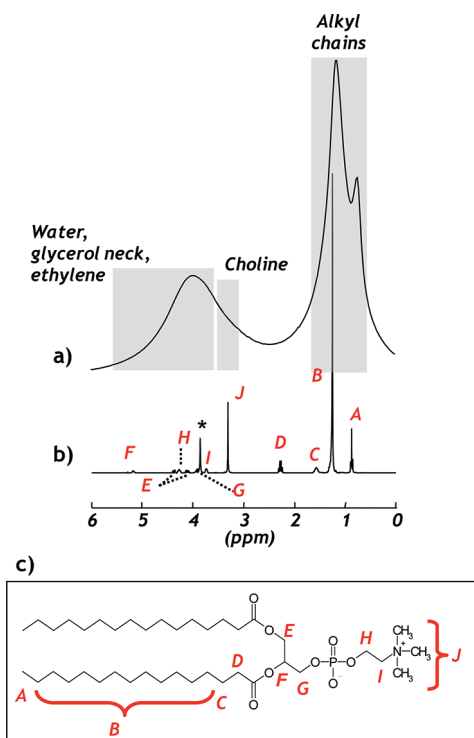
Figure 4. (a) Single pulse ^1\text{H} MAS ( \nu_{\text{MAS}} = 5\text{ kHz} ) spectrum of liposils and assignment of the principal regions. (b) Assigned ^1\text{H} spectrum of DPPC in \text{CDCl}_3 (see Figure S9 of the SI), (c) schematic representation of DPPC with atoms labeling. * denotes residual water in \text{CDCl}_3 .
