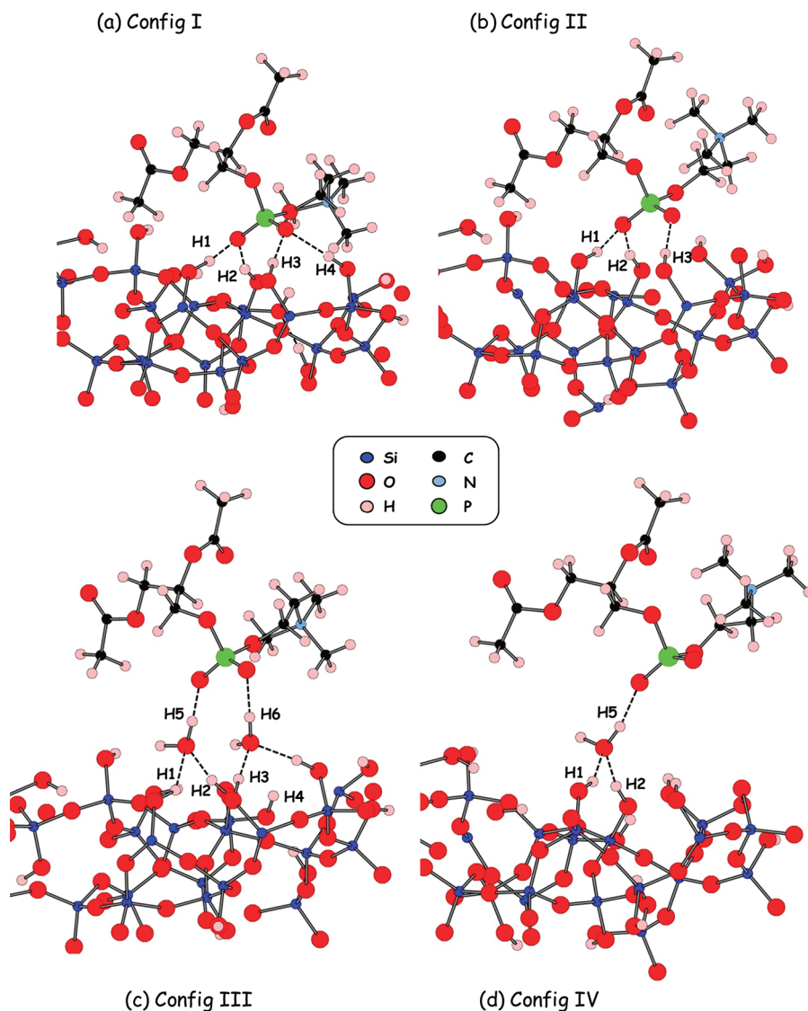
Figure 7. Representation of the configurations I, II, III, and IV obtained through geometry optimization (see the Experimental Section).
