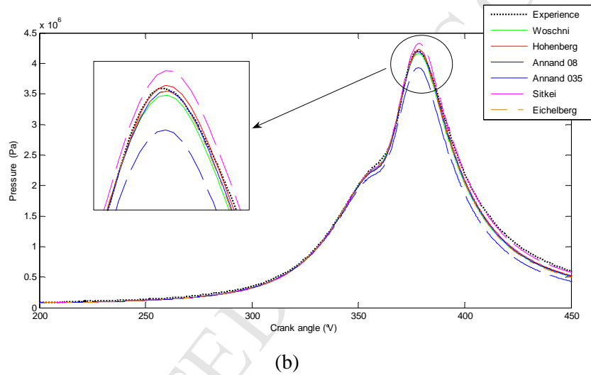
Fig. 5. Pressure comparison for different correlations within two cases: (a) \Phi=1, \alpha=9^\circ c.a, Full load (b) \Phi=1, \alpha=9^\circ c.a, Partial load
