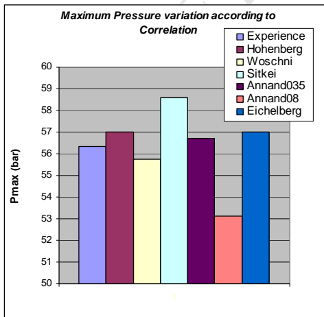
Fig. 6. Maximum Pressure comparison for different correlations within two cases: (a) \Phi=1, \alpha=9^\circ c.a, Full load (b) \Phi=1, \alpha=9^\circ c.a, Partial load
