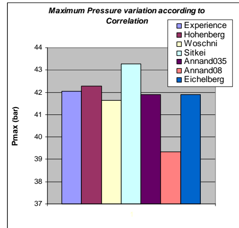
Fig. 6. Maximum Pressure comparison for different correlations within two cases: (a) \Phi=1, \alpha=9^\circ c.a, Full load (b) \Phi=1, \alpha=9^\circ c.a, Partial load
