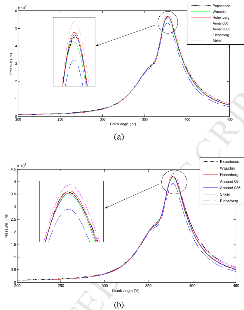
Fig. 5. Pressure comparison for different correlations within two cases: (a) \phi=1, \alpha=9^\circ c.a, Full load (b) \phi=1, \alpha=9^\circ c.a, Partial load
