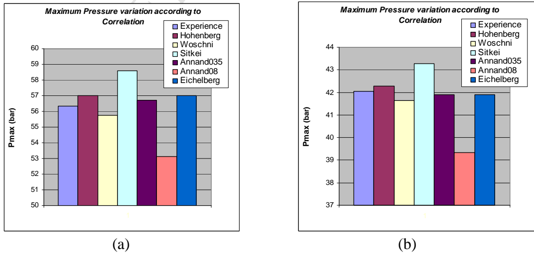
Fig. 6. Maximum Pressure comparison for different correlations within two cases: (a) \phi=1, \alpha=9^\circ c.a, Full load (b) \phi=1, \alpha=9^\circ c.a, Partial load
