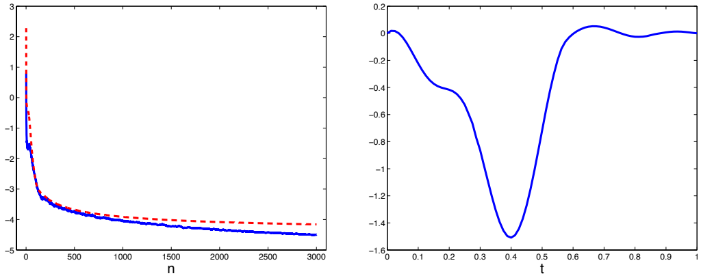
FIGURE 7. \beta = 0 : T = 3.5 , \Delta x = \Delta t = 1/80 - Left : \log_{10} of E_h(\mathbf{y}_h^n) ( dashed line ) and \log_{10}(\|\mathbf{g}_h^n\|_{\mathcal{A}_0}) ( full line ) vs. the iteration n of the conjugate gradient algorithm ; Right : Trace y_{1h}(\xi = 1, t) vs. t \in (0, T)
