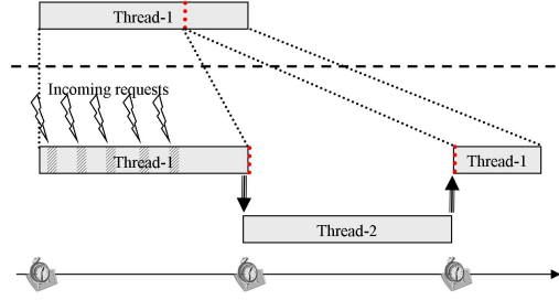
Fig. 3. Normal (up) and curtailed (down) execution of a thread
