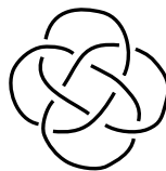
Figure 1. Knot topology for 8_{18} , based on a diagram from ref. [26].
