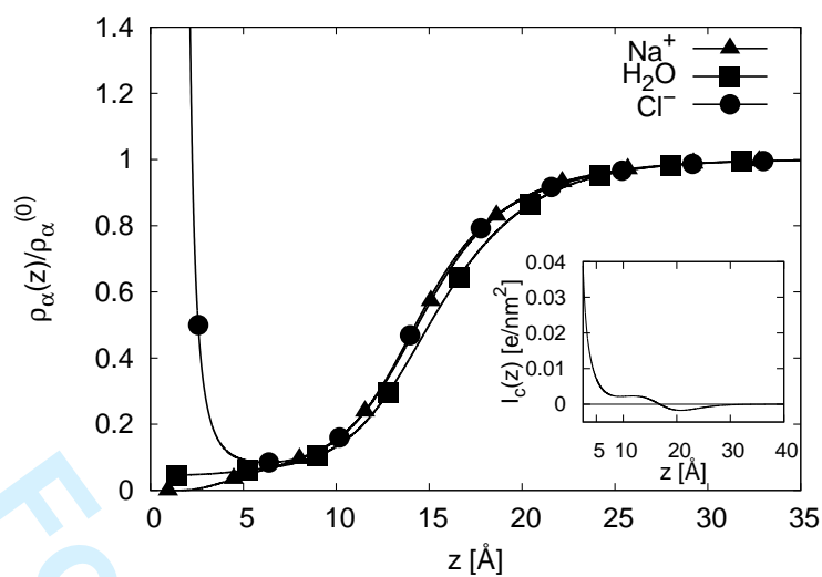
Figure 4: Density profiles of 1M NaCl at liquid-vapour coexistence near a hard wall carrying a surface charge \sigma^* = +0.0087 . T^* = 0.75 , \epsilon(z) is the CM function defined by ( 37). The inset shows the total amount of charge per unit area I_c(z) contained between 0 and z (including the substrate charge).
