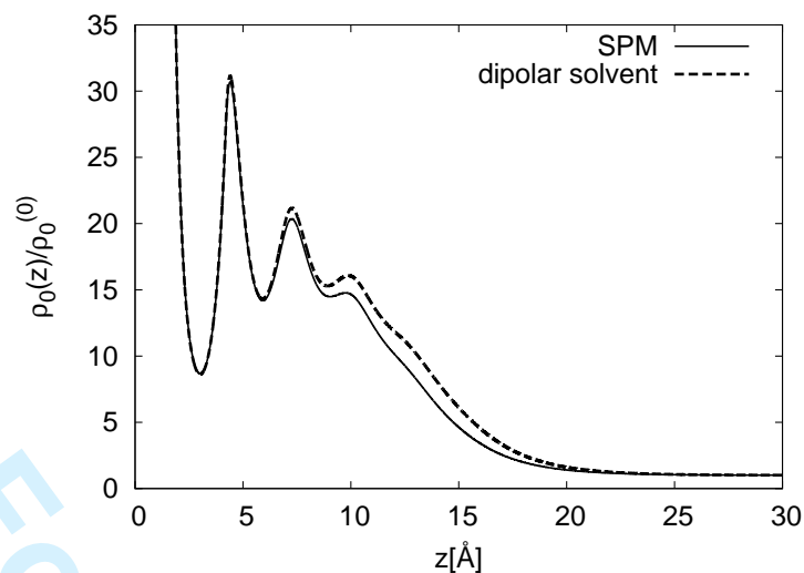
Figure 6: Solvent density profiles at coexistence (gas branch) compared for the SPM (with CM permittivity (37)) and the “civilized” solution model. The NaCl concentration in the corresponding liquid phase is 0.1M. The vapour is in contact with a wall carrying a surface charge density \sigma^* = +0.022 and exerting an exponential attraction with an inverse range parameter k_w = 1.8 . The temperature T^*=0.743 and the reduced dipole moment m^*=0.75 . Both systems are close to a second order wetting transition.
