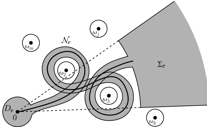
Figure 2.1 - A \nu -sectorial region
