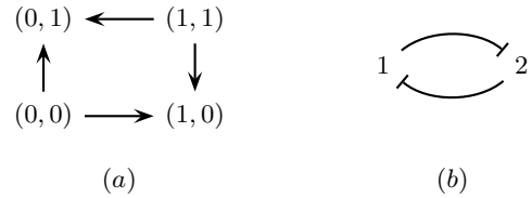
Fig. 1. (a) Asynchronous dynamics: the states of a system consisting in two variables 1 (horizontal axis) and 2 (vertical axis) are pictured; an arrow from state x to state \bar{x}^i means that f_i(x) \neq x_i . (b) The regulatory graph G(f)(x) , which turns out not to depend on x . Edges represent activations or inhibitions and are respectively denoted by arrows \rightarrow and T-end notation \dashv , which are more standard in biological literature than \xrightarrow{+} , \xrightarrow{-} .
