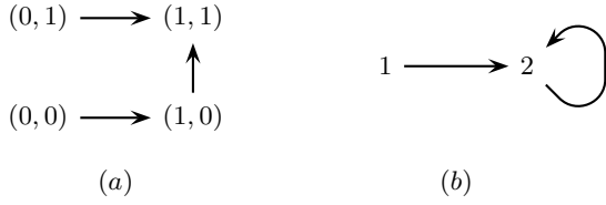
Fig. 4. (a) An example of dynamics with a globally minimal circuit (loop on 2), two 2-fixed points, but a single global fixed point. (b) The regulatory graph.
