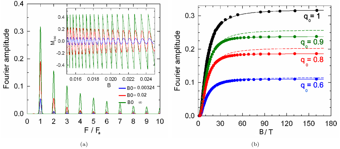
Figure 5. (Color on-line) (a) Fourier spectra of the dHvA oscillations of a linear chain of compensated orbits, for various values of the magnetic breakdown field B_0 . The effective masses are m_e = 1 and m_h = 2.5 , and \Delta = 1 (see text). F_a = 7/2 is the fundamental frequency for this model. (b) B/T dependence of the first harmonic amplitude A_a for various values of the tunneling probability (hence of the magnetic field). Solid symbols come from numerical resolution of the semiclassical spectrum, which fall onto the solid lines corresponding to the Lifshits-Kosevich approximation given by Eq. 19 including contributions of zero area orbits. Dashed lines correspond to the first order term l = 1 in Eq. 19 or equivalently to Eq. 3.
