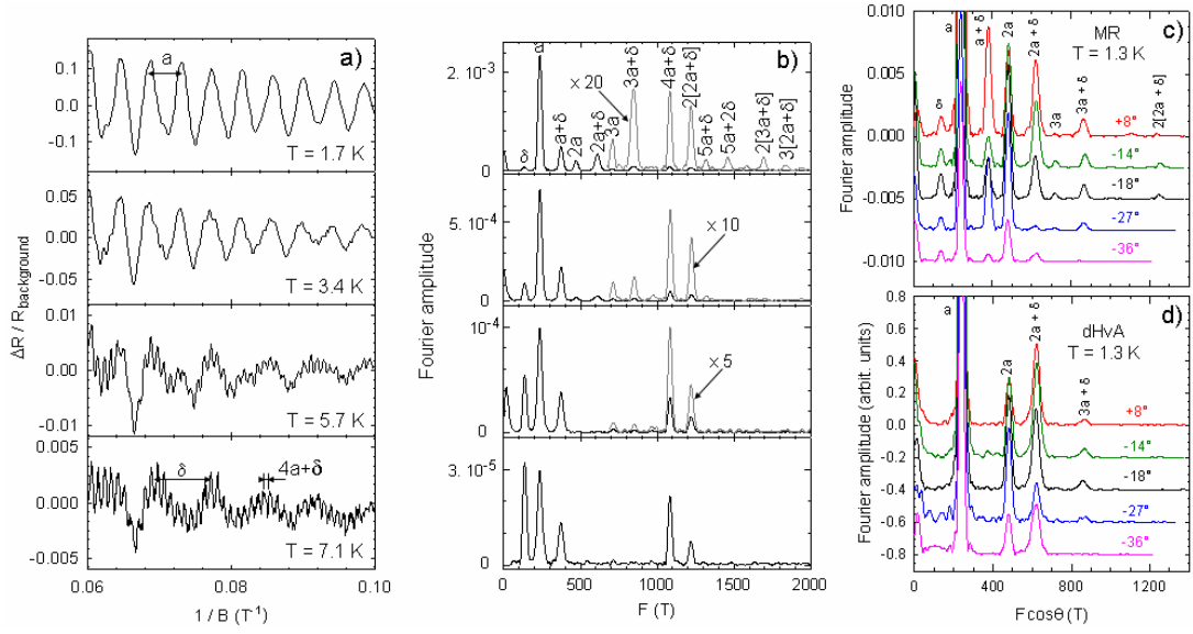
Figure 4. (Colour on-line) (a) Oscillatory part of the magnetoresistance and (b) corresponding Fourier spectra of (\text{ET})_8[\text{Hg}_4\text{Cl}_{12}(\text{C}_6\text{H}_5\text{Br})_2] at various temperatures [58]. Fourier spectra of (c) magnetoresistance and (d) de Haas-van Alphen oscillations for various directions of the magnetic field [59]. Data in (c) and (d) have been measured simultaneously. Labels a and \delta correspond to closed and forbidden orbits, respectively, depicted in Fig 1(d). Contrary to magnetoresistance oscillations spectra which exhibits forbidden frequency combinations, all the dHvA components are accounted for by the Falicov-Stachowiak semiclassical model.
