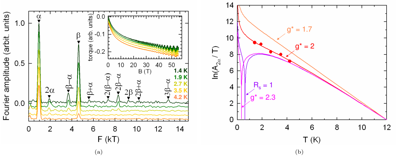
Figure 3. (Color on-line) (a) Fourier analysis in the field range 35-55.3 T of the magnetic torque data reported in the insert. Solid triangles are marks calculated with F_\alpha(\theta = 0) = 0.944 kT and F_\beta(\theta = 0) = 4.60 kT. Data have been shifted down from each other by a constant amount. (b) Temperature dependence (mass plot) of the 2\alpha amplitude. Symbols are data deduced from torque measurements of Fig. 3(a) at 48.3 T. Solid lines are deduced from Eq. 13 with m_\alpha = 1.81 , m_\beta = 3.52 , T_D = 0.79 K and B_0 = 35 T. Spin damping factor (see Eq. 8) is either neglected ( R_p^s = 1 , p = 1 to 3) or accounted for by various g^* values. All the data are normalized to their values at 12 K.
