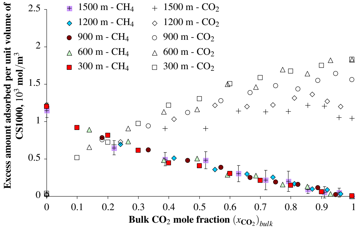
Figure 8: Excess amounts isotherms for the adsorption of the CO 2 -CH 4 mixture in CS1000 for the various geological depths considered. For sake of clarity we displayed the uncertainties for one of the curves only.
