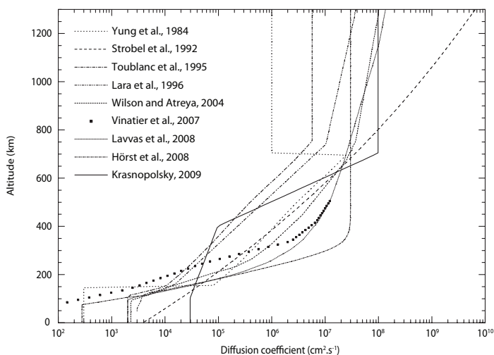
Fig. 1. Eddy diffusion profiles from various photochemical models (Yung et al. 1984; Strobel et al. 1992; Toublanc et al. 1995; Lara et al. 1996; Wilson & Atreya 2004; Vinatier et al. 2007; Lavvas et al. 2008; Hörst et al. 2008; Krasnopolsky 2009).
