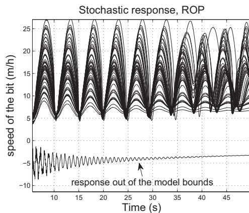
Figure 4: \delta = 0.03 . Nonparametric model. 50 Monte Carlo simulations of the ROP.
