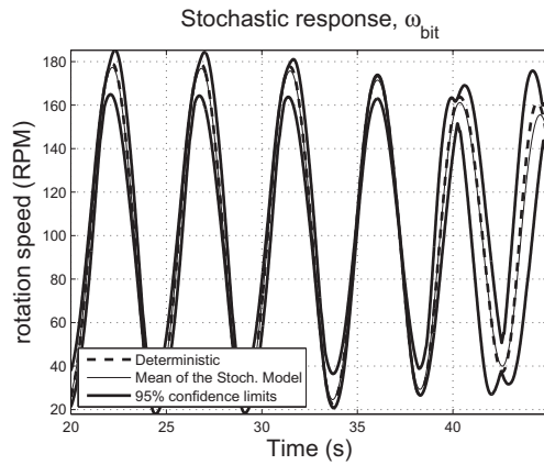
Figure 2: \delta = 0.01 . Nonparametric model, rotation speed of the bit, 95% envelope.
