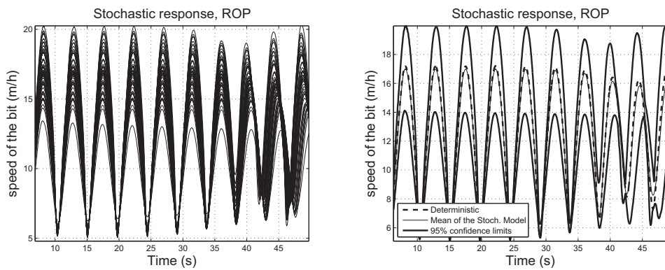
Figure 1: \delta = 0.01 . Nonparametric model, rate-of-penetration, ROP. Left: 50 Monte Carlo simulations. Right: 95% envelope.
