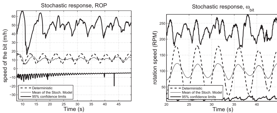
Figure 3: \delta = 0.1 . Nonparametric model, 95% envelope. Left: rate-of-penetration, ROP. Right: rotation speed of the bit.
