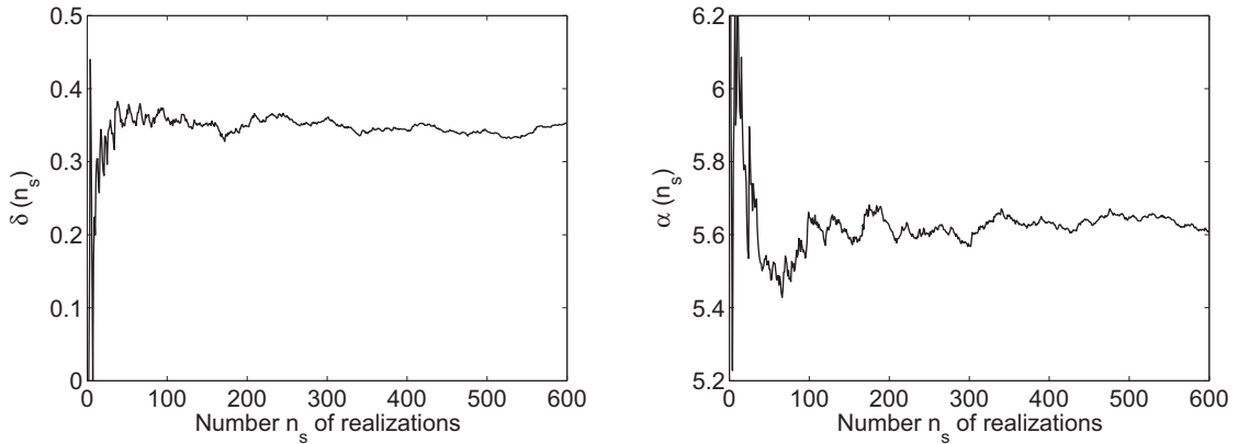
Figure 6. Graph of n_s \mapsto \delta(n_s) (left figure) and graph of n_s \mapsto \alpha(n_s) (right figure).
