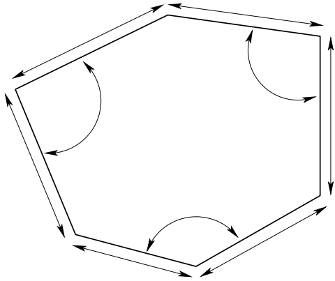
Figure 1: Rigid GCS
