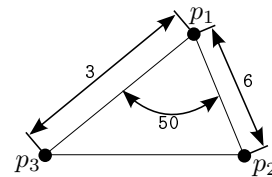
Figure 5: A 2D sketch of a rigid triangle.
