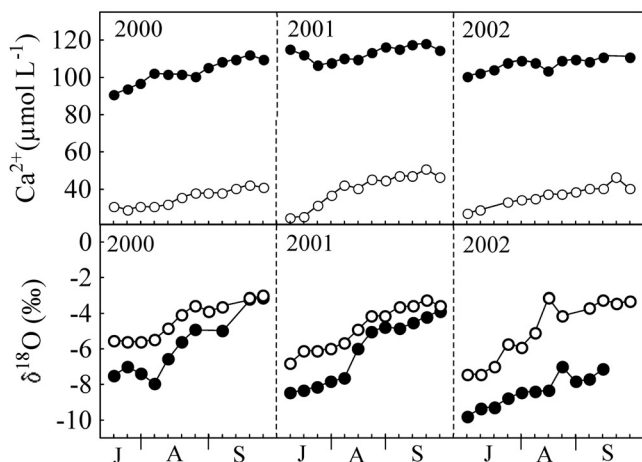
Figure 3. Dynamics of (top) calcium concentration (Ca) and (bottom) oxygen isotopic signature ( \delta^{18}\text{O} ) in La Caldera Lake (solid symbols) and Río Seco Lake (open symbols) during the ice-free periods of 2000, 2001, and 2002.
