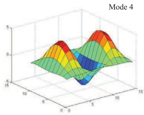
Figure 5. First four modes of the flexible boundary plate, k=0.75 , 120 boundary modes, 10 clamped modes
