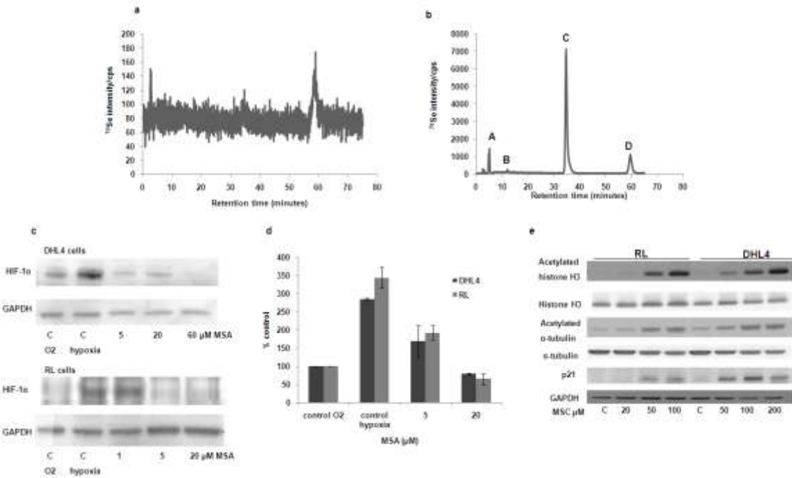
Figure 2 (a) Representative chromatogram of control DHL4 cells (b) Representative chromatogram demonstrating intracellular Se species generated after exposure of DHL4 cell to 20 \mu\text{M} MSA for 2 hours Peak A is MSC, peak B is SLM, peak C is dimethylselenide and peak D is S-methylselenogluthatione (c) HIF1 \alpha expression in DHL4 and RL cells exposed to hypoxia and MSA for 24 hours (d) VEGF levels in the supernatant of DHL4 and RL cells exposed to hypoxia and MSA for 24 hours (e) protein acetylation and p21 expression in RL and DHL4 cells exposed to MSC.
