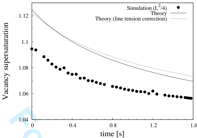
Figure 4. Time evolution of the vacancy supersaturation, c_{\infty}(t)/c_0 , for the initial total loops area L^2/4 . The lines are predictions of the KBS model for different line tension approximations. The solid line corresponds to Eq. (16) where the line tension is \mu b/R . The dashed line corresponds to Eq. (18) where the line tension is given by Eq. (17) with r_c = 1.5 \text{ \AA} .
