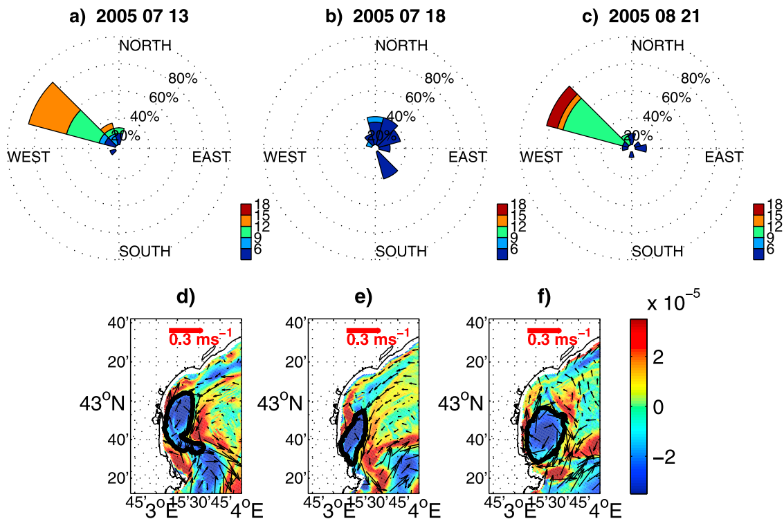
Figure 6. Time sequences of the evolution of the eddy A1_2005. Wind rose representation (intensity and frequency) at station Leucate on (a) 2005/07/11 to 13, (b) 2005/07/16 to 18, and (c) 2005/08/19 to 21, with the location and extension of the fan sector indicating of a wind direction and its percentage and colors representing wind intensity. Relative vorticity ( s^{-1} ) computed at 20 m depth and current velocity fields corresponding to the same depth on (d) 2005/07/13, (e) 2005/07/18, and (f) 2005/08/21. Black contours show the eddy identification issued from the wavelet analysis.
