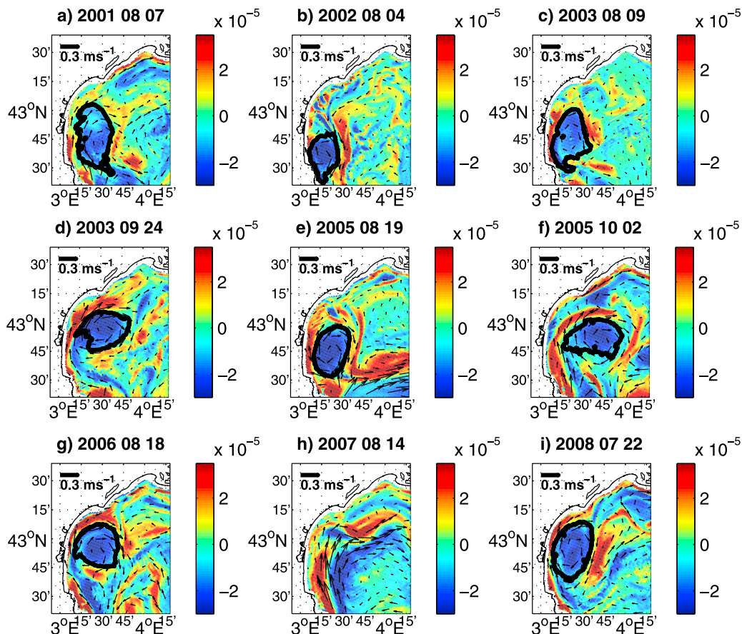
Figure 4. Snapshot of the modeled relative vorticity [ s^{-1} ] and current velocity at 20 m depth. The black contours issued from the wavelet analysis show the 8 long-life anticyclonic eddies once they are well-developed: (a) A1_2001, (b) A1_2002, (c) A1_2003, (d) A2_2003, (e) A1_2005, (f) A2_2005, (g) A1_2006, and (i) A1_2008. (h) The circulation over the western part of the shelf.
