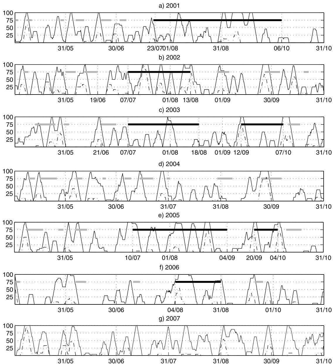
Figure 7. Temporal evolution of northwesterly expressed as a percentage of all wind, with a 3 day moving average, (solid line, northwesterly intensity \geq 8 \text{ ms}^{-1} ; dashed line, \geq 14 \text{ ms}^{-1} ) from May 1 to October 31 for each year. The presence of ‘long-life’ eddies is indicated by a horizontal black thick line and the ‘short-life’ eddies’ presence is indicated by a gray thick line.
