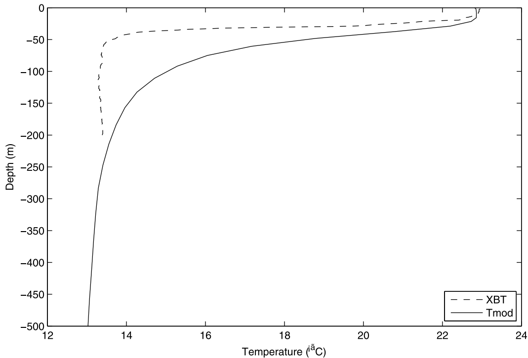
Figure 3. Vertical profile of temperature ( ^{\circ}\text{C} ) simulated (solid line) and measured (dashed line) by XBT at cross location in Figure 2.
