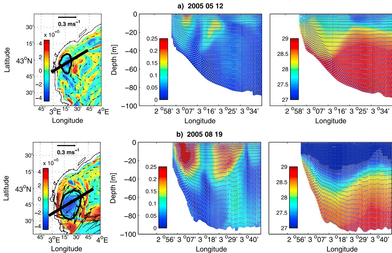
Figure 9. (left) Relative vorticity at 20 m depth, current velocity fields and eddy contour, where the black line marks the eddy cross-section; (middle) vertical transect of current intensity [ \text{ms}^{-1} ]; and (right) vertical transect of density for (a) May 12 and (b) August 19, in 2005.
