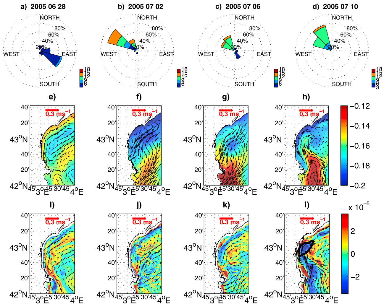
Figure 5. Time sequences of the generation process of the eddy A1 2005 with 4 days of interval. Wind rose representation (intensity and frequency) at station Leucate on (a) 2005/06/26 to 28, (b) 2005/06/30 to 07/02, (c) 2005/07/04 to 06, and (d) 2005/07/08 to 10, with colors representing wind intensity. Sea surface height and current velocity field at 5 m depth on (e) 2005/06/28, (f) 2005/07/02, (g) 2005/07/06, and (h) 2005/07/10. (i–l) Relative vorticity ( s^{-1} ) computed at 20 m depth and current velocity fields corresponding to the same depth at the same dates as Figures 5e–5h. Black contour in Figure 5l shows the eddy identification issued from the wavelet analysis.
