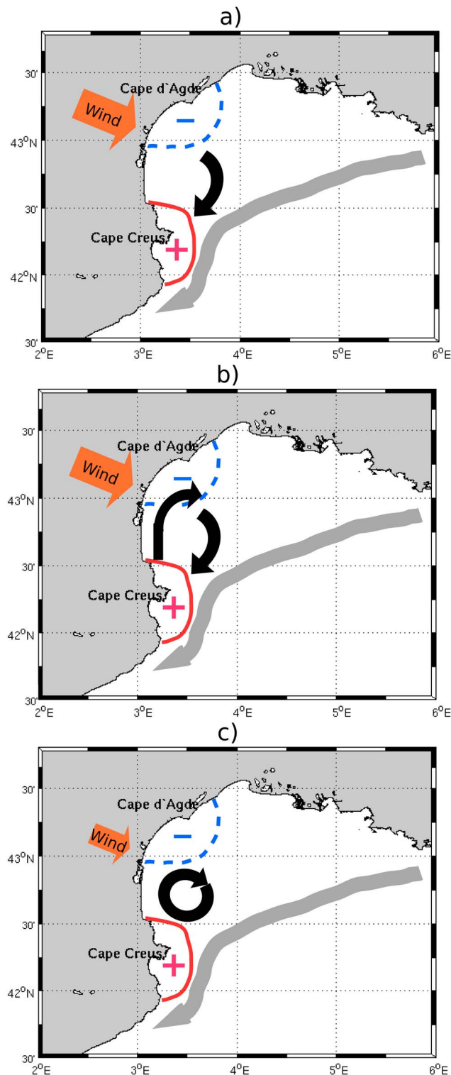
Figure 10. Schematic of anticyclonic eddy generation process. Wind-forcing is indicated by the orange arrows; also shown are sea surface level (red plus or blue minus zones), surface currents (black thick arrow), and NC (gray thick line).
