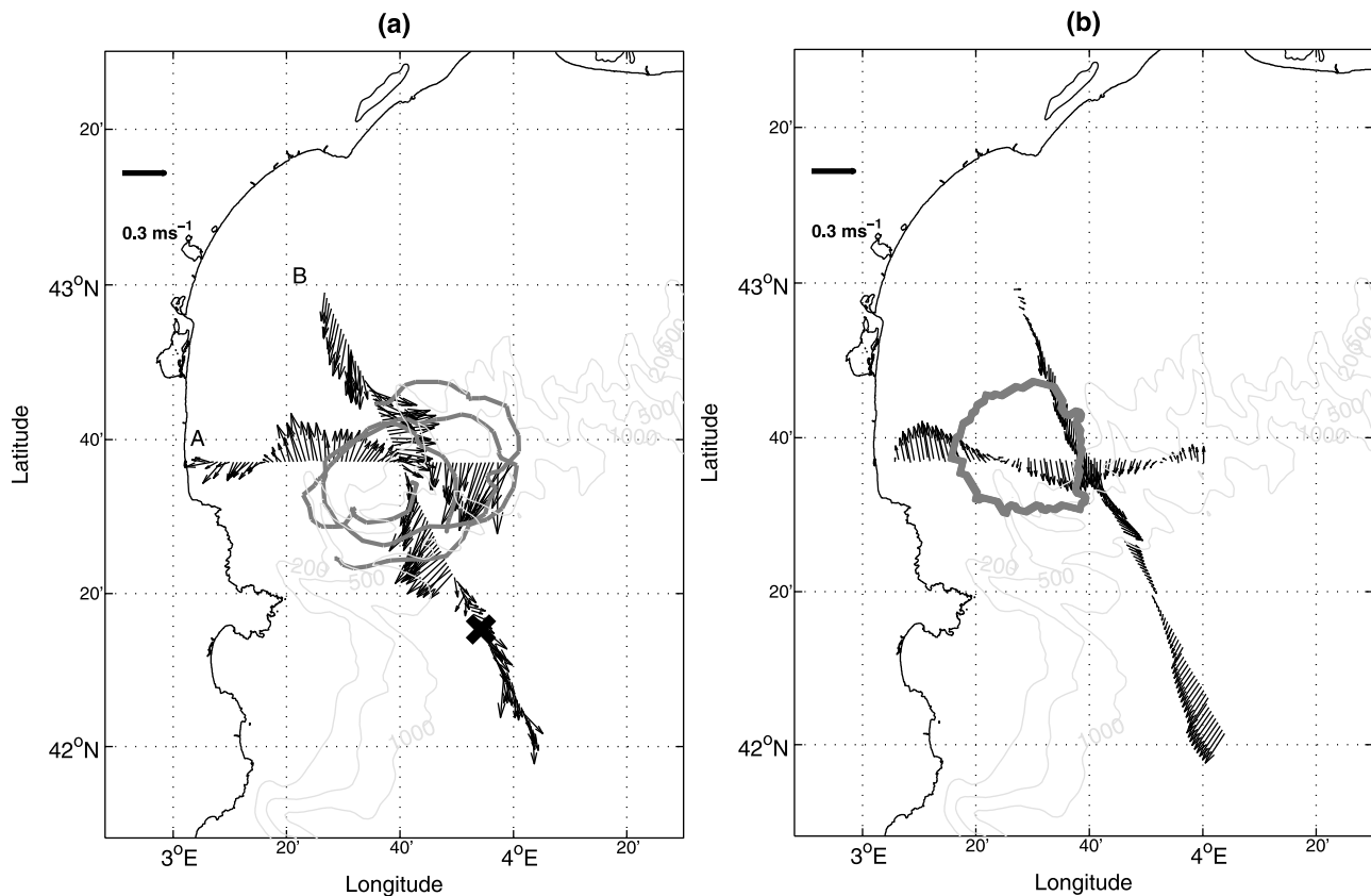
Figure 2. Comparison of the horizontal current field ( \text{ms}^{-1} ) at 15 m depth. (a) ADCP measured current along transect A on Sept. 1, and along transect B on Sept. 5, 2008. Dark gray contours represent the trajectories of two drifters from Sept. 5 to Sept. 11; the thick cross indicates XBT station. (b) Simulated current averaged from Sept. 1 00:00 to Sept. 2 00:00 along transect A and from Sept. 5 00:00 to Sept. 6 00:00 along transect B. Dark gray contour represents the eddy identification issued from the wavelet analysis on Sept. 10.
