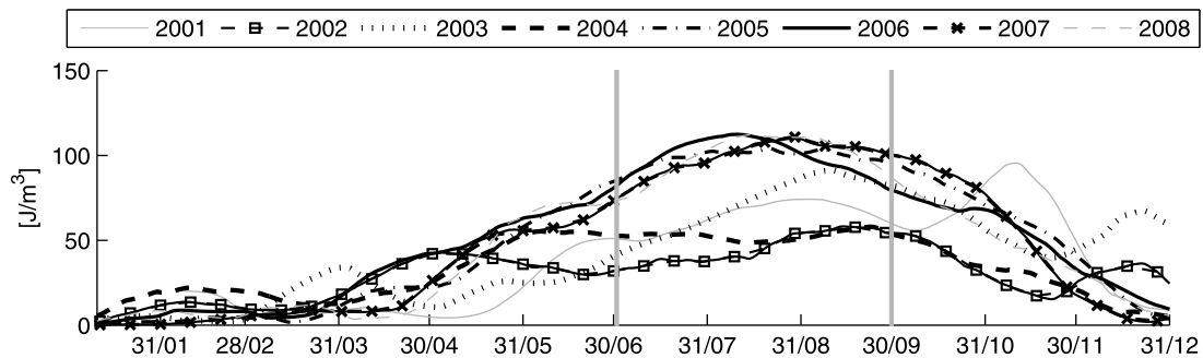
Figure 8. Time series of 30 day moving averaged absolute potential energy anomaly [ \text{J}/\text{m}^3 ] over the western part of the GoL for the upper 100 m depth for the years 2001–2008.
