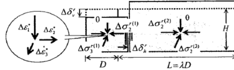
Fig. 13. Residual stress increments due to permanent strain increments in the "two-block" system
