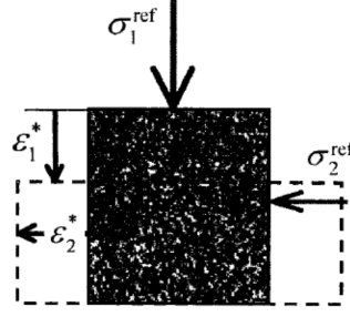
Fig. 9. Maximum stresses and associated permanent strains
