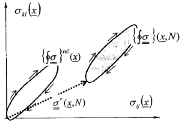
Fig. 3. Reference and current stress cycles at point \underline{x}
