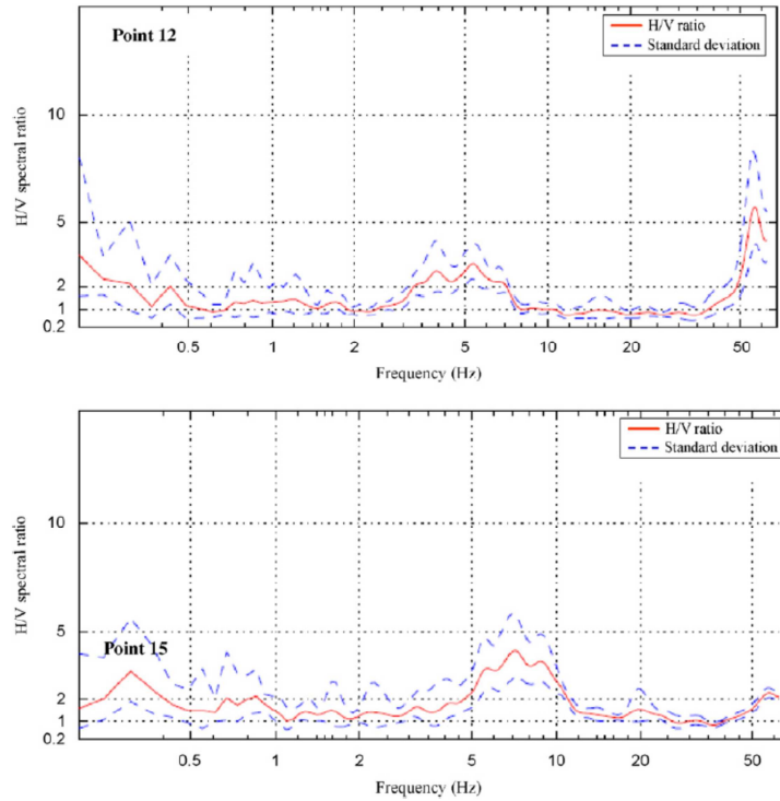
Fig. 8. Example of H/V ratio from ambient noise at points 12 and 15 close to the residence LAG.
