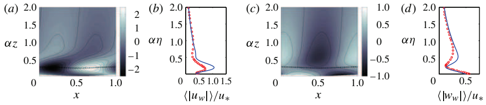
FIGURE 12. The same as figure 10, with c/U_* = 7.8 . The critical layer, where U_0(z_c) = c , is marked by a broken line.
