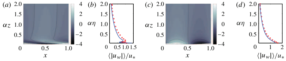
FIGURE 13. The same as figure 10, with c/U_* = 22 .
