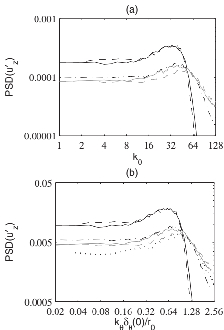
FIG. 16. PSDs normalized by u_j of fluctuating velocity u'_z at r=r_0 as functions (a) of wave number k_\theta and (b) of k_\theta \delta_\theta(0)/r_0 for — Jetring256, - - - Jetring256drdz, - - - - Jetring512, gray solid line: Jetring1024dz, and gray dashed line: Jetring1024drdz at z=0.4r_0 and for \cdots\cdots Jetring1024drdz 2\delta_\theta at z=0.8r_0 .
