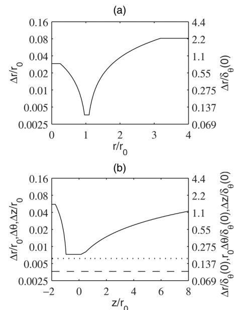
FIG. 4. Representation, in logarithmic scales, of the mesh spacings in Jetring1024drdz2 \delta_\theta : (a) \Delta r as a function of r/r_0 , (b) — \Delta z , - - - \Delta r , and \cdots \cdots r_0 \Delta \theta at r=r_0 . The mesh spacings are normalized by r_0 or \delta_\theta(0) as in Figs. 2 and 3.
