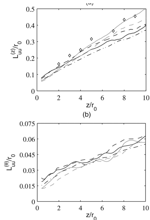
FIG. 17. Variations of the integral length scales (a) L_{uu}^{(z)} and (b) L_{uu}^{(\theta)} , calculated from velocity u'_z at r=r_0 for — Jetring256, - - - Jetring256drdz, - - - - Jetring512, gray solid line: Jetring1024dz, and gray dashed line: Jetring1024drdz. Measurements: \diamond Fleury et al. (Ref. 49) for a Mach 0.9 jet at Re_D=7.7 \times 10^5 .
