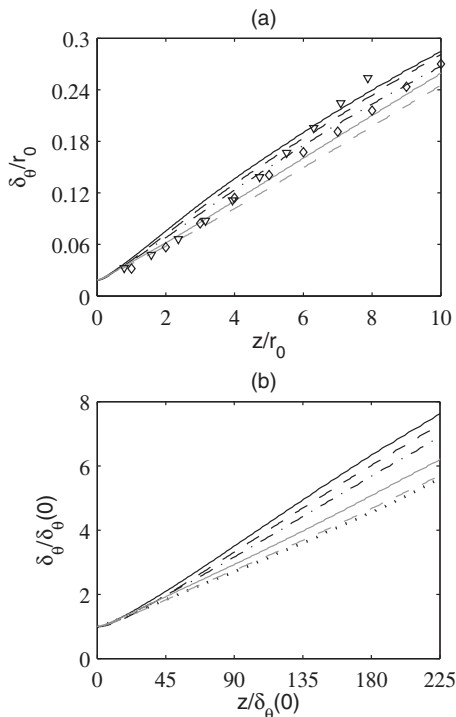
FIG. 18. Variations of shear-layer momentum thickness \delta_\theta normalized (a) by r_0 and (b) by \delta_\theta(0) for — Jetring256, - - - Jetring256drdz, - · - · - Jetring512, gray solid line: Jetring1024dz, gray dashed line: Jetring1024drdz, and ···· Jetring1024drdz2 \delta_\theta . Measurements: \nabla Husain and Hussain (Ref. 13) for an initially turbulent axisymmetric shear layer and \diamond Fleury et al. (Ref. 49) for a Mach 0.9 jet at Re_D=7.7 \times 10^5 .
