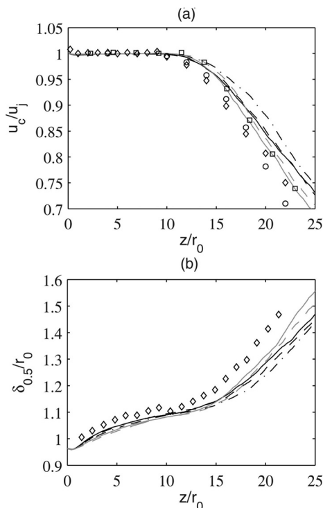
FIG. 22. Variations (a) of centerline mean axial velocity u_c and (b) of jet half-width \delta_{0.5} for — Jetring256, --- Jetring256drdz, - - - - Jetring512, gray solid line: Jetring1024dz, gray dashed line: Jetring1024drdz. Measurements for Mach 0.9 jets at Re_D \geq 5 \times 10^5 : \circ Lau et al. (Ref. 50), \square Arakeri et al. (Ref. 17), and \diamond Fleury et al. (Ref. 49).
