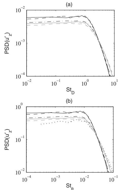
FIG. 15. PSDs normalized by u_j of axial fluctuating velocity u'_z at r=r_0 as functions (a) of St_D=fD/u_j and (b) of St_\theta=f\delta_\theta(0)/u_j for — Jetring256, - - - Jetring256drdz, - · - · - Jetring512, gray solid line: Jetring1024dz, and gray dashed line: Jetring1024drdz at z=0.4r_0 and for ····· Jetring1024drdz2 \delta_\theta at z=0.8r_0 .
