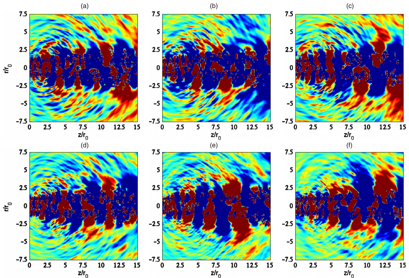
FIG. 10. (Color online) Snapshots in the (z, r) plane of fluctuating pressure p - p_a obtained by LES for (a) Jetnoise256, (b) Jetring256, (c) Jetring256drdz, (d) Jetring512, (e) Jetring1024dz, and (f) Jetring1024drdz. The color scale ranges from levels of -100 to 100 Pa.
