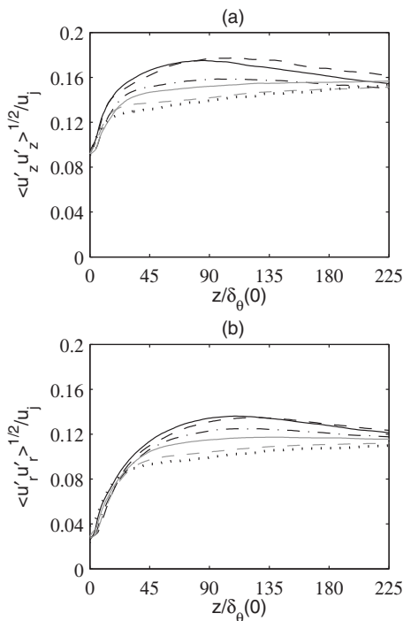
FIG. 20. Variations of the peak rms values of velocities (a) u'_z and (b) u'_r as functions of z/\delta_\theta(0) for — Jetring256, --- Jetring256drdz, - - - - Jetring512, gray solid line: Jetring1024dz, gray dashed line: Jetring1024drdz, and \cdots\cdots Jetring1024drdz 2\delta_\theta .
