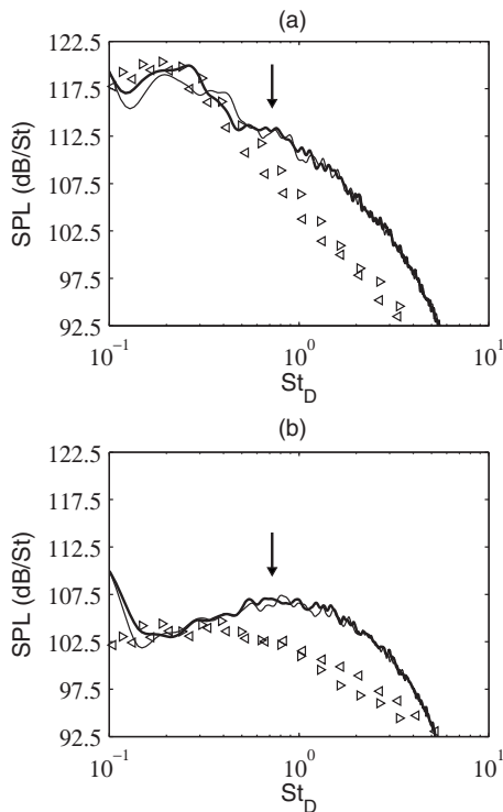
FIG. 14. Sound pressure levels (SPL) obtained at 60r_0 from the jet exit as functions of St_D=fD/u_j at the angles of (a) 30^\circ and (b) 90^\circ for — (thick line) Jetnoise256 and — (thin line) Jetring256. The arrows indicate the frequency determined using St_\theta=f\delta_\theta(0)/u_j=0.0065 . Measurements for jets at Re_D \geq 7.8 \times 10^5 : \triangleleft Tanna (Ref. 51) and \triangle Bogey et al. (Ref. 52).
