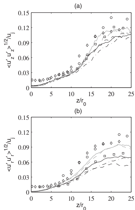
FIG. 23. Variations of centerline rms values of fluctuating velocities (a) u'_z and (b) u'_r for — Jetring256, --- Jetring256drdz, - - - - Jetring512, gray solid line: Jetring1024dz, and gray dashed line: Jetring1024drdz. Measurements for Mach 0.9 jets at Re_D \geq 5 \times 10^5 : \square Arakeri et al. (Ref. 17), \circ Lau et al. (Ref. 50), and \diamond Fleury et al. (Ref. 49).
