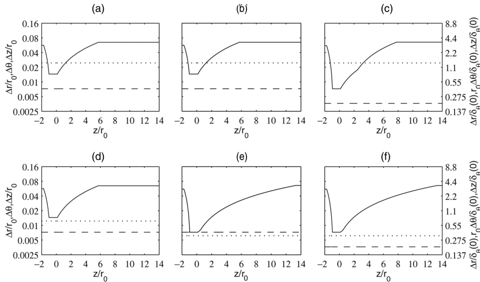
FIG. 3. Representation, in logarithmic scales, of the mesh spacings, — \Delta z , - - - \Delta r , \cdots \cdots r_0 \Delta \theta , at r=r_0 in (a) Jetnoise256, (b) Jetring256, (c) Jetring256drdz, (d) Jetring512, (e) Jetring1024dz, and (f) Jetring1024drdz. The mesh spacings are normalized by r_0 or \delta_\theta(0) as in Fig. 2.
