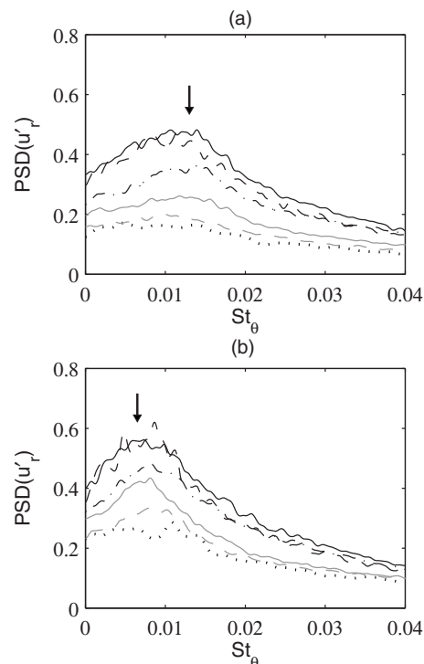
FIG. 21. PSDs normalized by u_j of radial velocity u'_r at r=r_0 as functions of St_\theta = f\delta_\theta(0)/u_j for — Jetring256, --- Jetring256drdz, - - - - Jetring512, gray solid line: Jetring1024dz, and gray dashed line: Jetring1024drdz (a) at z=1.5r_0 and (b) at z=3r_0 and for \cdots\cdots Jetring1024drdz 2\delta_\theta (a) at z=3r_0 and (b) at z=6r_0 . The arrows indicate (a) St_\theta=0.013 and (b) St_\theta=0.0065 .
