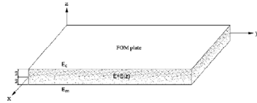
Fig. 1. Geometry of the functionally graded plate.
