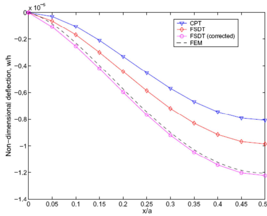
Fig. 9. Variation profile of deflection for various model, E_c/E_m = 6 , p = 6 , a/h = 10 , e_c/e_{ft} = 2 .
