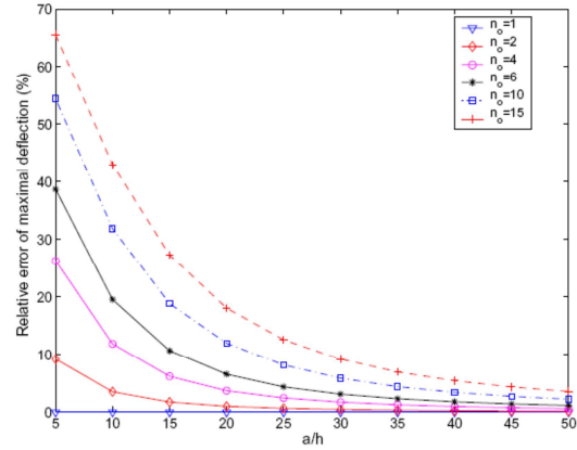
Fig. 8. Relative error of maximal deflection according to the ratio of length-thickness, e_c/e_{ft} = 2 , p = 6 .
