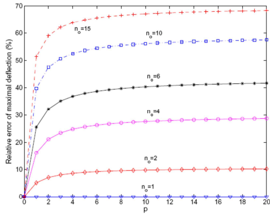
Fig. 7. Relative error of maximal deflection in terms of p , e_c/e_{ft} = 2 , a/h = 5 .
