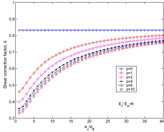
Fig. 6. Variation of the shear factors in terms of the ratio of e_c/e_{ft} , E_c/E_m = 6 .
