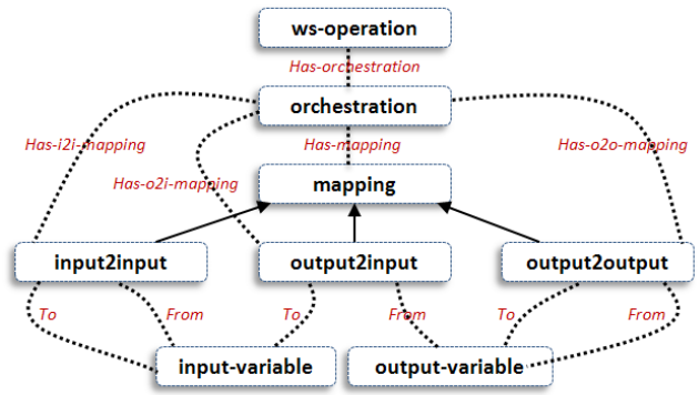
Figure 2. Semantic model for describing the composition of image processing tools as workflow
