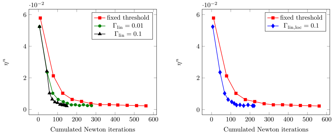
Figure 4: Error estimator \eta^n c.f. (5.2) as a function of the cumulated Newton iterations at each time step (time steps are identified by markers). Global stopping criterion (4.1) ( left ), local stopping criterion (7.3) ( right )
