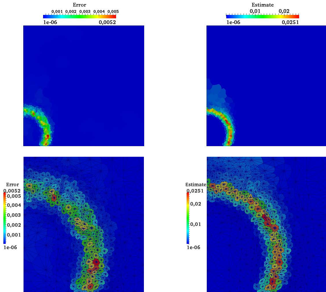
Figure 7: Actual ( left ) and estimated ( right ) error distribution for \Gamma_{\text{lin}} = \Gamma_{\text{reg}} = 0.1 , adaptive Algorithm 4.1, entire domain ( top ), interface ( bottom )
