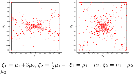
Fig. 7.8: Sample set patterns for different type of parametrized functions with singular behavior on two crossing line with different slopes.
