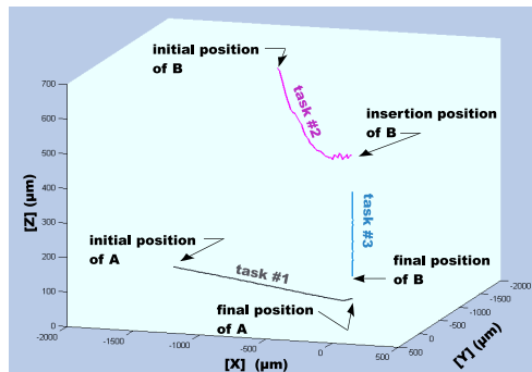
Fig. 8. Part trajectories.
