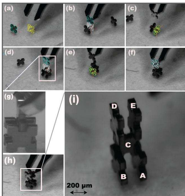
Fig. 9. Assembly of five parts on three levels.
