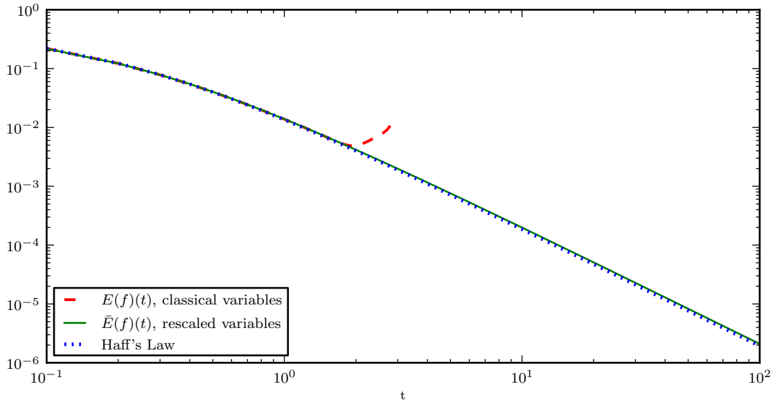
FIGURE 4. Comparison of the global inhomogeneous cooling process in original and scaled variables ( \varepsilon = 0.1 ).
