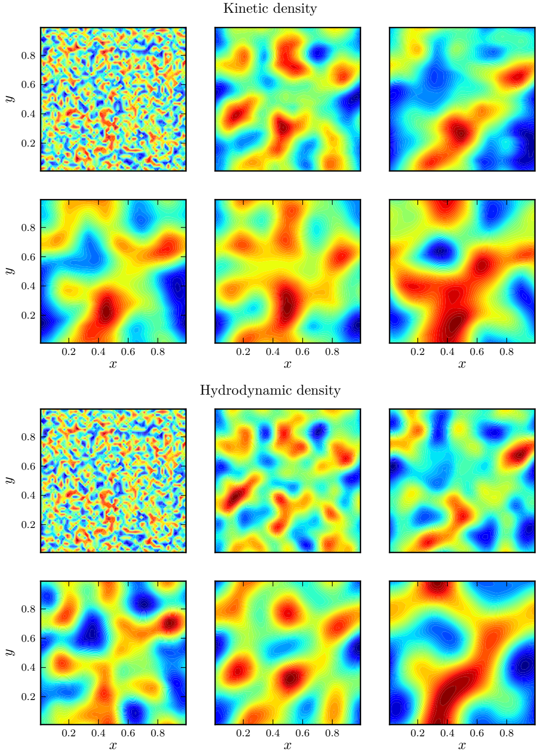
FIGURE 7. Contour plot of the density given by the simplified granular gases model (top) and the dissipative Euler system (bottom), at time t = 0, 0.25, 0.5, 1, 5 and 10 . High values are displayed in red, low in blue.
