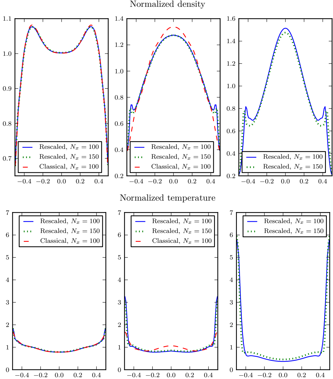
FIGURE 6. Normalized density \rho(t, x)/\bar{\rho} and temperature T(t, x)/\bar{T}(t) of the shear flow problem computed in classical and rescaled variables, at time t = 0.25, 0.75 and 2 .
