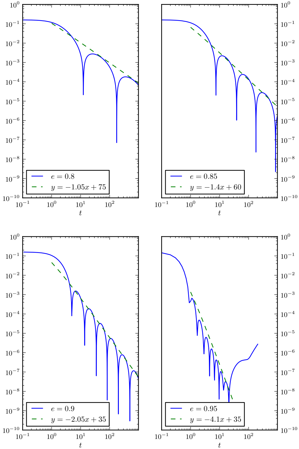
FIGURE 5. Return to equilibrium of \mathcal{L}(t) = \|\rho - 1\|_{L^1} .
