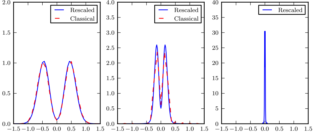
FIGURE 3. Comparison of the first marginal f^{(1)} of the solution to (6.1) computed in classical (dashed line) and rescaled variables (solid line), at time t = 0.3, 1 and 20 .
