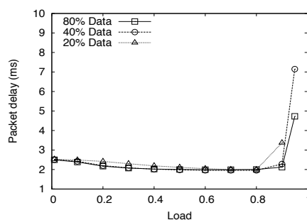
FIGURE 4: Mean packet delay of video flows.
