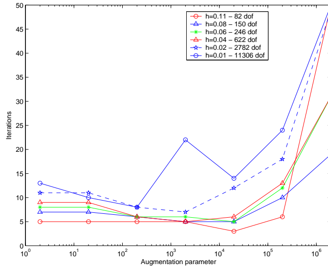
Figure 14: ( SSN ) influence of the augmentation parameter r for the disc with different mesh sizes.
