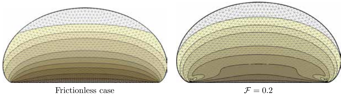
Figure 3: case(a) , the Von Mises criterion on the deformed disc meshed with P_2 isoparametric FEM in frictional contact with a rigid foundation (with Getfem [26]).
