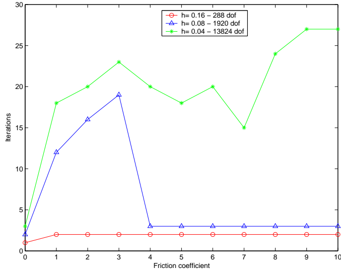
Figure 13: ( SSN ) influence of the friction coefficient for the torus with different mesh sizes.
