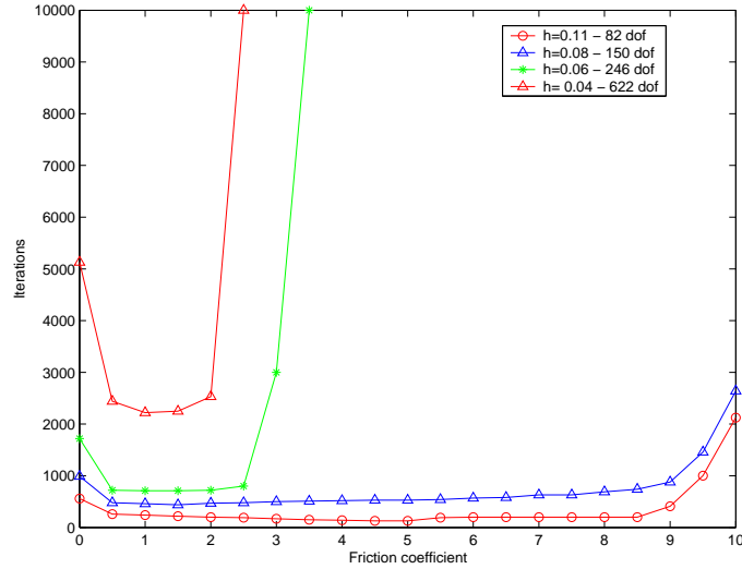
Figure 11: (SOR) influence of the mesh size for the disc (with \omega = 1.5 and nodal strategy).
