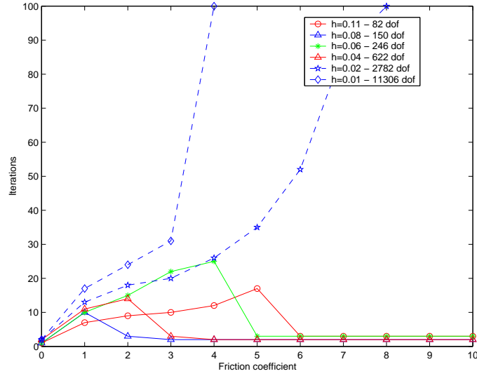
Figure 9: ( FPT ) influence of the friction coefficient for the disc with different mesh sizes.
