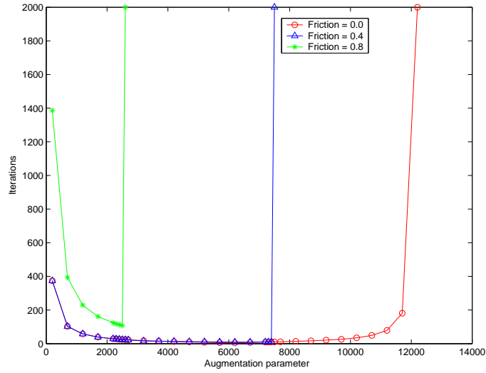
Figure 6: ( FPS ) influence of the augmentation parameter r for the torus with different values of the friction coefficient.
