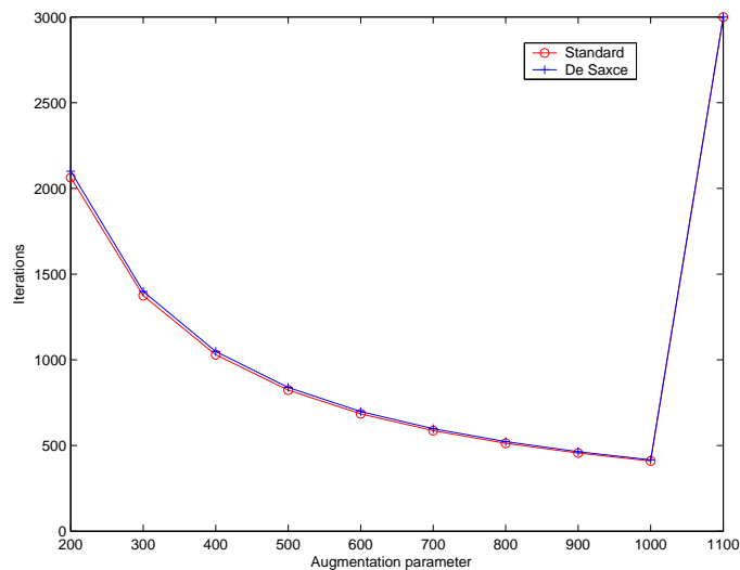
Figure 18: (FPS) comparison of the De Saxcé formulation with the standard one for the disc.
