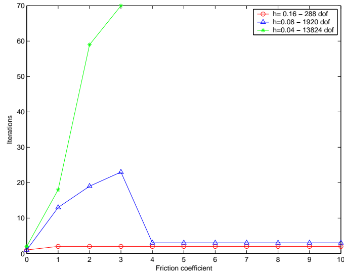
Figure 10: ( FPT ) influence of the friction coefficient for the torus with different mesh sizes.
