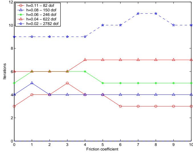
Figure 12: ( SSN ) influence of the friction coefficient for the disc with different mesh sizes.
