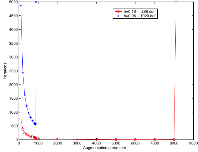
Figure 8: (FPS) influence of the augmentation parameter r for the torus with different mesh sizes.
