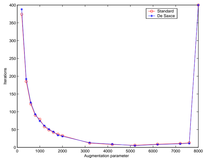
Figure 19: (FPS) comparison of the De Saxcé formulation with the standard one for the torus.
