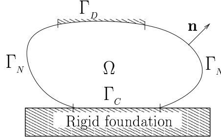
Figure 1: linearly elastic body \Omega in frictional contact with a rigid foundation.
