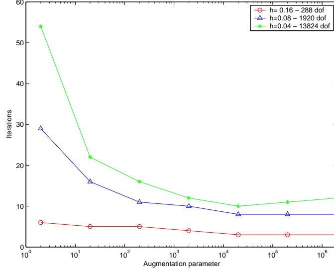
Figure 15: ( SSN ) influence of the augmentation parameter r for the torus with different mesh sizes.
