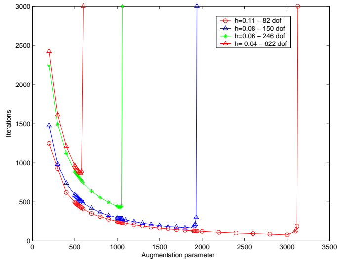
Figure 7: ( FPS ) influence of the augmentation parameter r for the disc with different mesh sizes.
