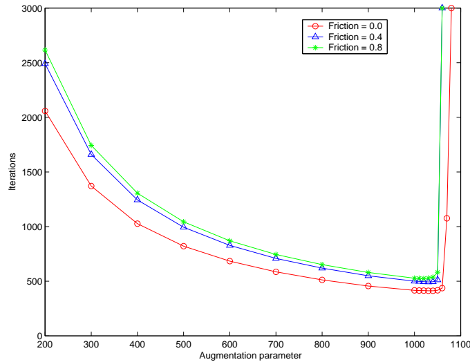
Figure 5: (FPS) influence of the augmentation parameter r for the disc with different values of the friction coefficient.
