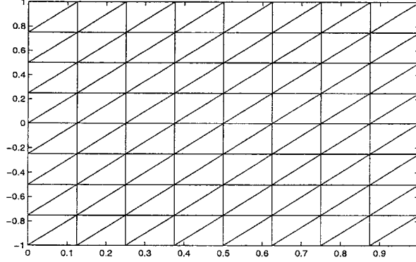
Fig. 3. Structured mesh of the domain \bar{\Omega} .
