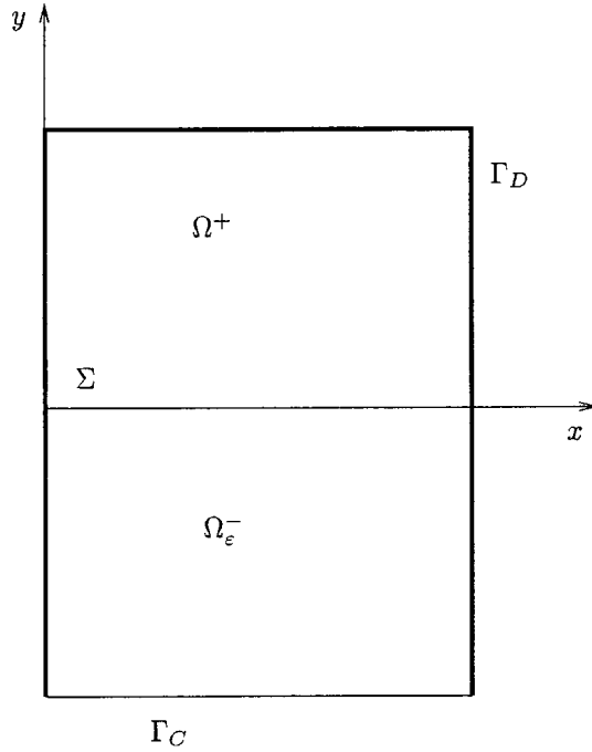
Fig. 2. Domain after change of variable.
