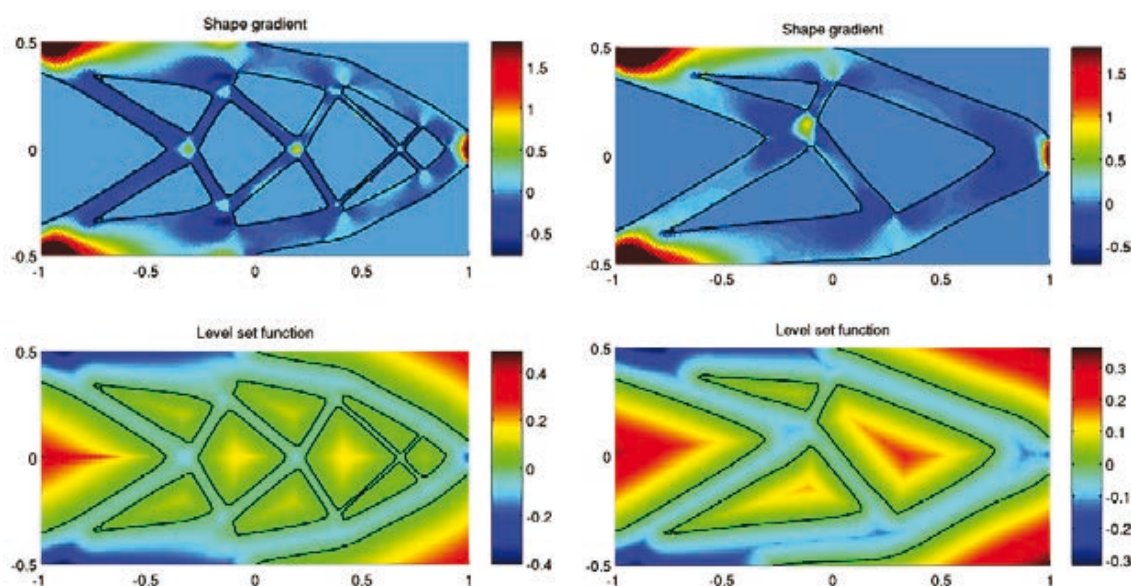
Figure 6. Optimal shape design in a 80 \times 160 mesh.
