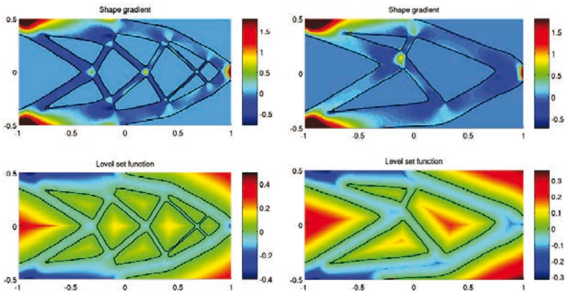
Figure 4. Fourth step (optimal design).
