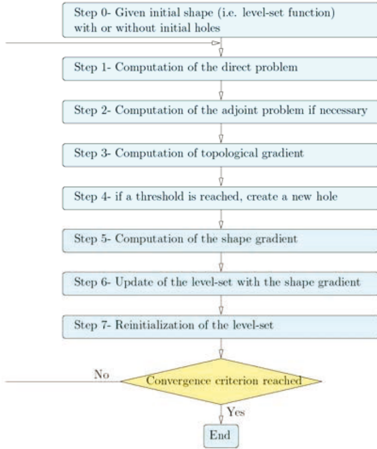
Figure 2. Structural optimization algorithm.
