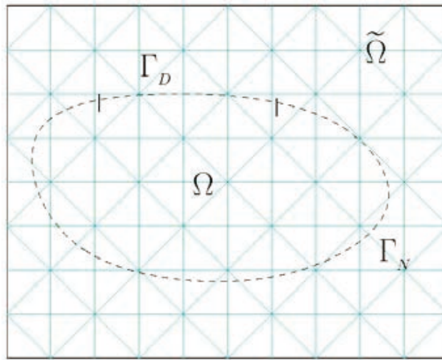
Figure 1. Example of a structured mesh.
