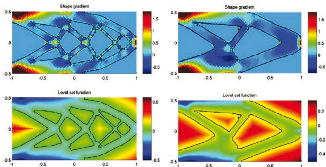
Figure 5. Optimal shape design in a 40 \times 80 mesh.
