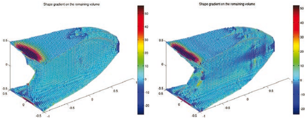
Figure 8. Fourth step (optimal shape).
