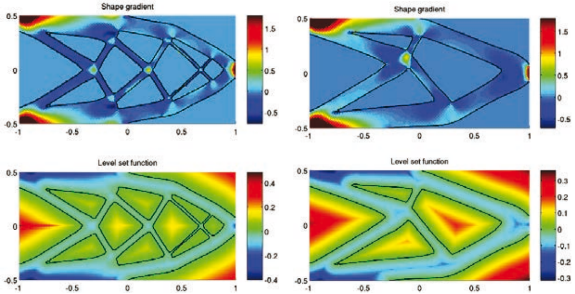
Figure 6. Optimal shape design in a 80 \times 160 mesh.
