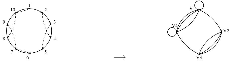
(a) A cyclic graph G and a partition \pi of its vertices
