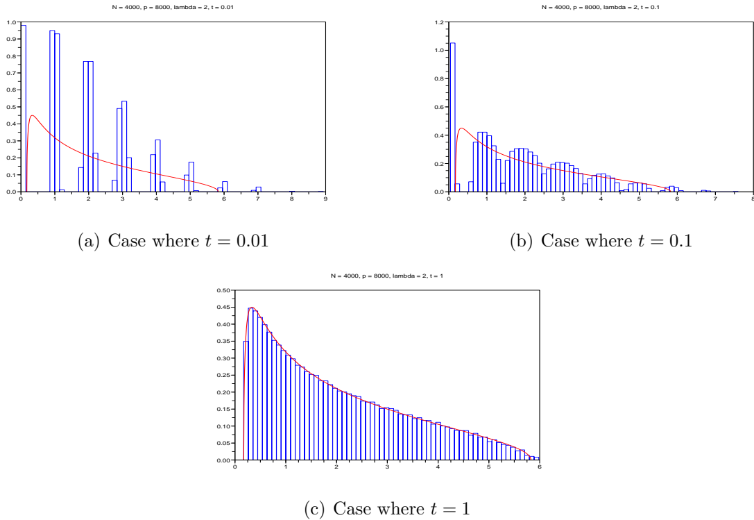
FIGURE 1. The empirical spectral distribution of the matrix M of (4) for N = 4 \cdot 10^3 , p = 8 \cdot 10^3 at several values of t . We see that this distribution, which is approximately the law P_{2,t} , is close to the Poisson law with parameter 2 for t close to zero, and that it converges to the Marchenko-Pastur law with parameter 2 (whose density is plotted by a smooth continuous line) as t grows.
