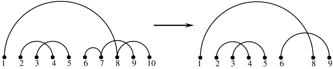
FIGURE 3. Illustration of the operation \pi \mapsto \text{thin}(\pi)
