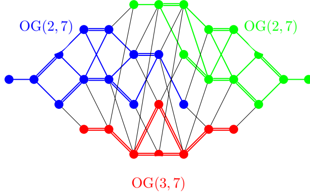
Figure 2: P_{\omega_1} -orbits in \text{OG}(3, 9)
