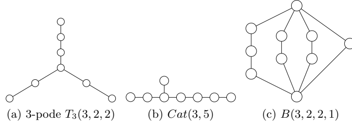
Figure 1: Examples of special graphs
