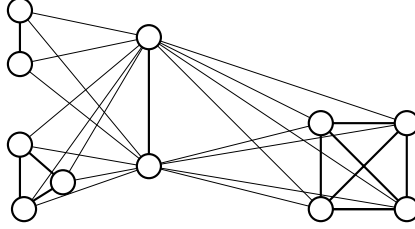
Figure 2: Graph K_2(2, 3, 4)
