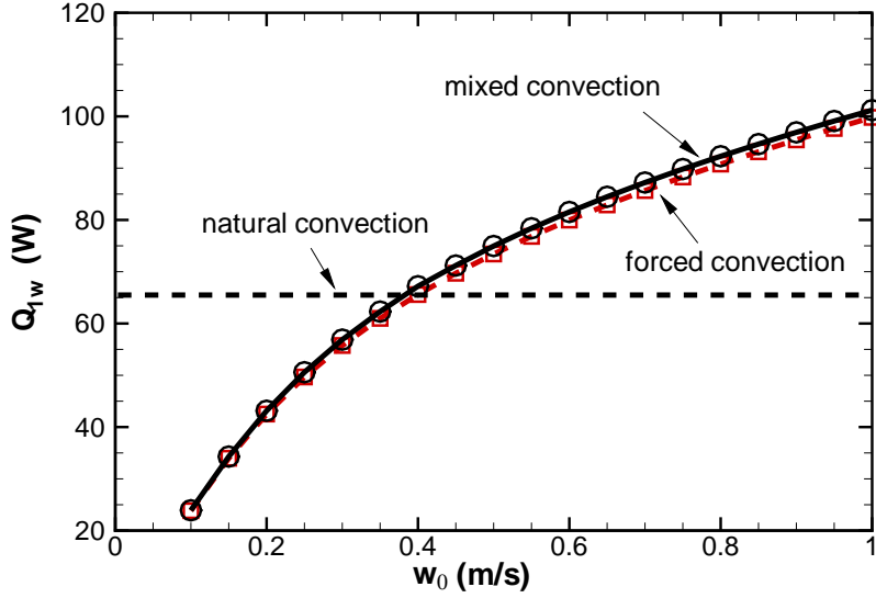
Fig. 5 Total heat flux transferred at one of the hot walls for forced and mixed convection according to the prescribed inlet velocity. The value for natural convection is also shown ( D = 2 \text{ cm} , H = 1 \text{ m} , \Delta T = 20 \text{ K} ).
