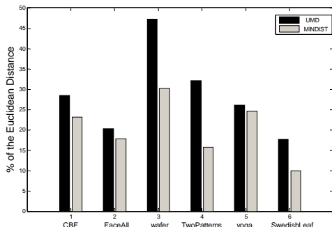
Figure 3: Comparison of the tightness of UMD with the tightness of MINDIST in 6 data sets and for alphabet size=3. The figure shows that UMD is tighter than MINDIST.
