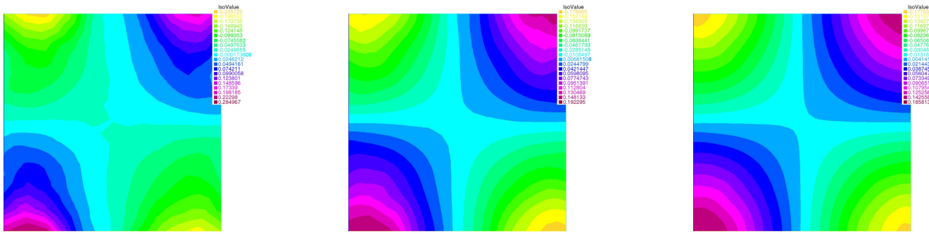
Figure 6: Adaptive computed pressure using the error indicator.
