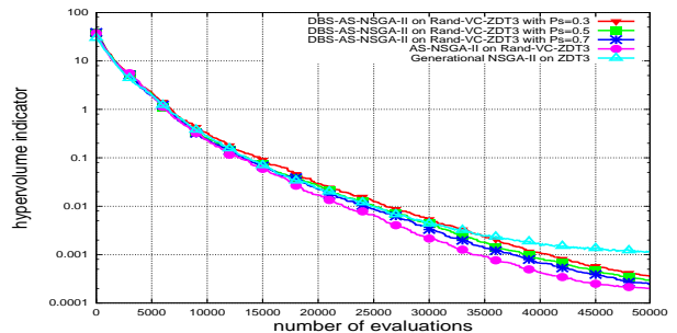
Figure 7: Evolution of average hypervolume indicator for DBS-AS-NSGA-II with different values of P_s on (plain) function ZDT3.
