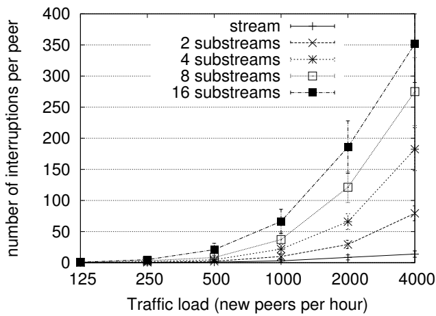
Fig. 15. Impact of the number of substreams on the interruptions.
