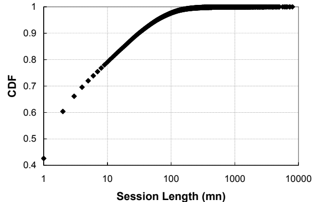
Fig. 1. Distribution of the peers' session length.
