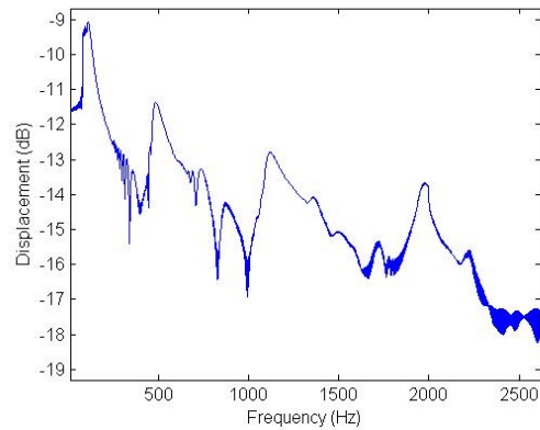
Figure 8. Transverse displacement of the middle of the beam (nonlinear mean model) as a function of frequency.
