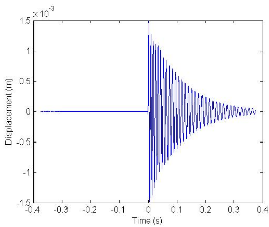
Figure 7. Transverse displacement of the middle of the beam (nonlinear mean model) as a function of time.
